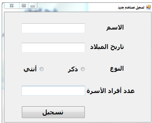
Figure (1-11) User interface to be designed
