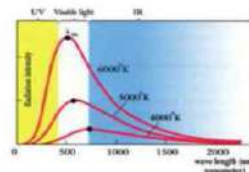
The wavelength at the peak is inversely proportional to temperature.
