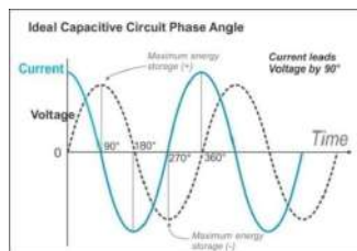
AC voltage lags AC current in a capacitor by 90^\circ
