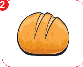
bun
