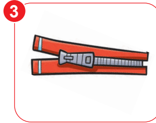
zip
